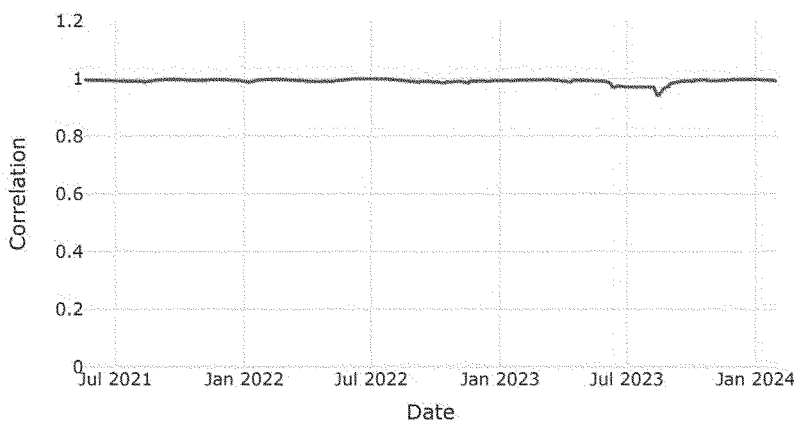
ETH spot and CME ETH futures daily returns
