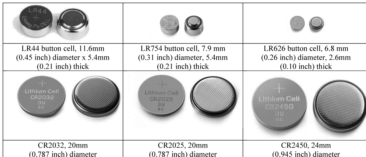
Figure 1. Example button cell and coin batteries.
