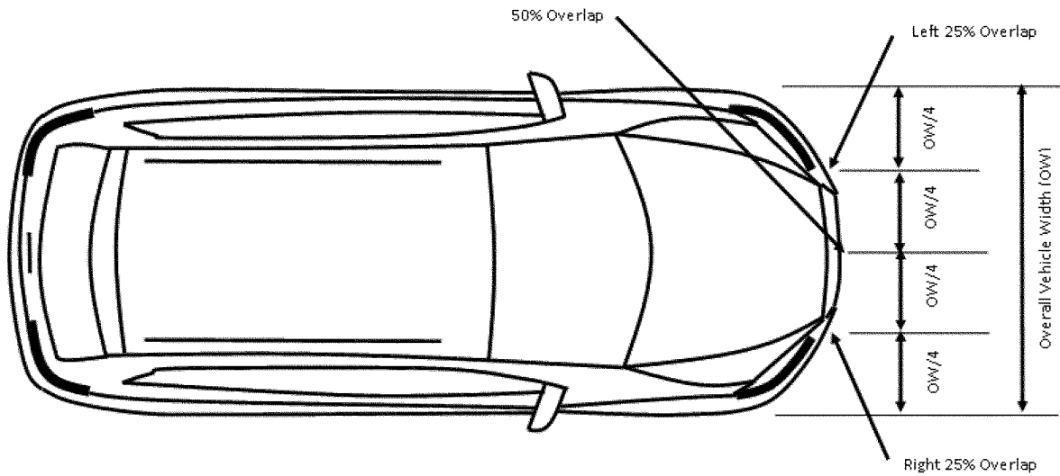
Figure 2 to § 571.127—Setup for Lead Vehicle Automatic Emergency Braking
