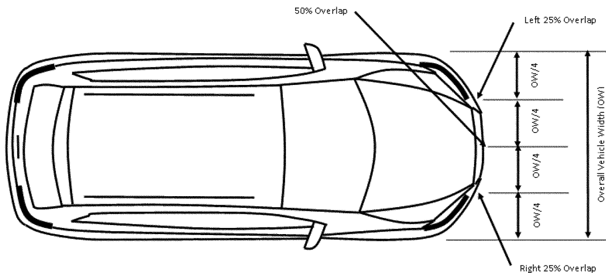
Figure 12: Vehicle Overlap
