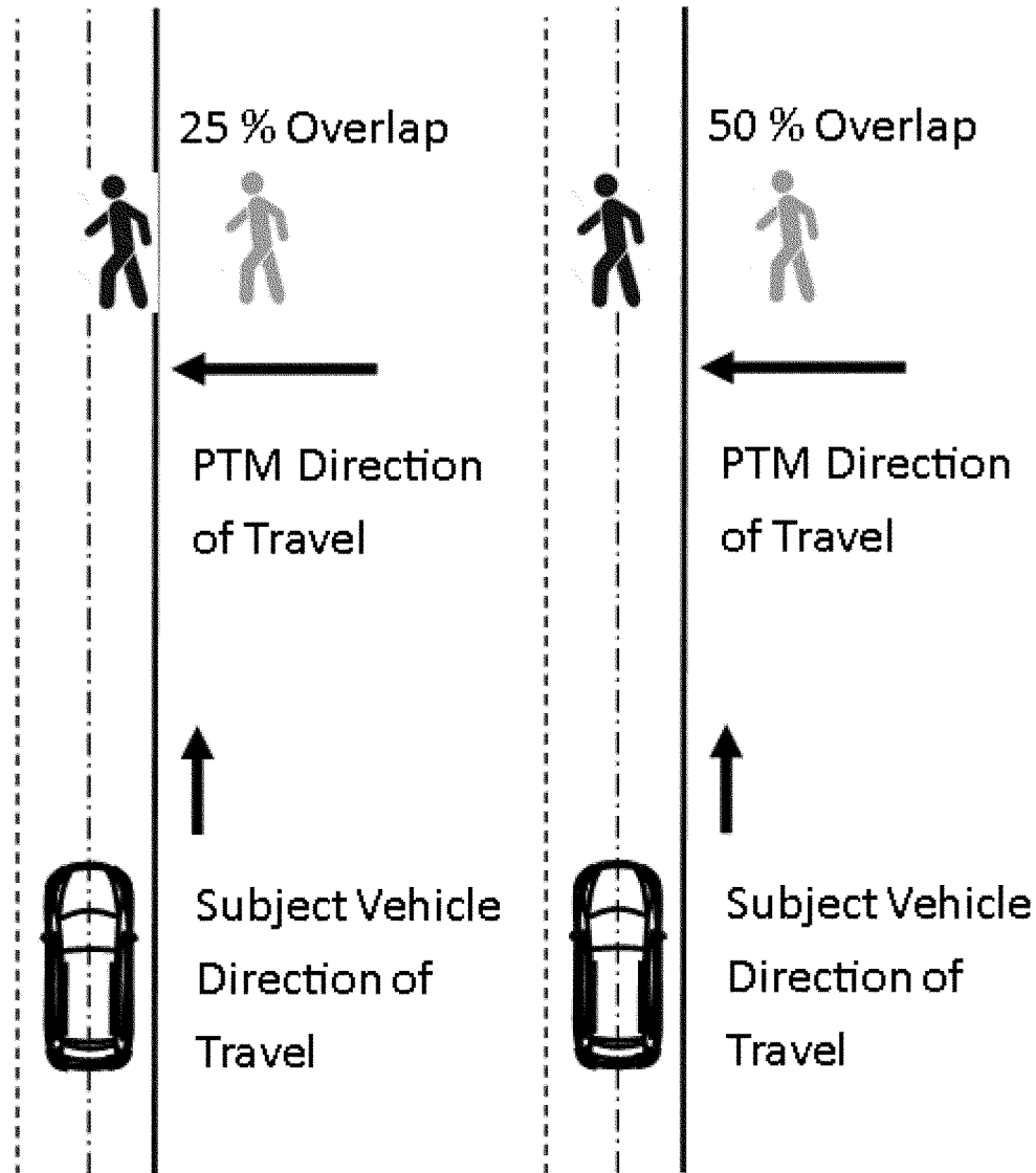
Figure 7: Pedestrian Crossing Path from the Right 25 and 50 Percent Overlap Basic Setup
