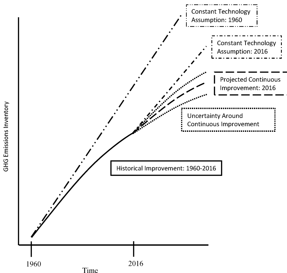
Figure VI-4 Illustration of different baselines relative to historical GHG emissions inventory
