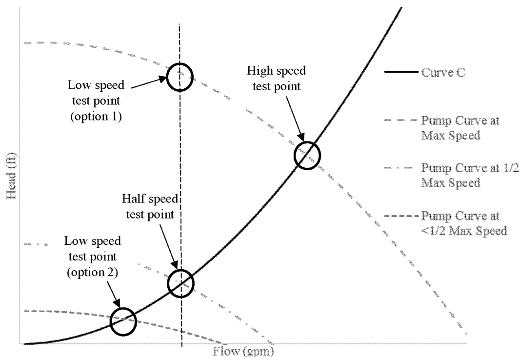
Figure III.4. Specified Load Points on Curve C at Maximum Speed for Two-Speed Self-Priming and Non-Self-Priming Pool Filter Pumps.
