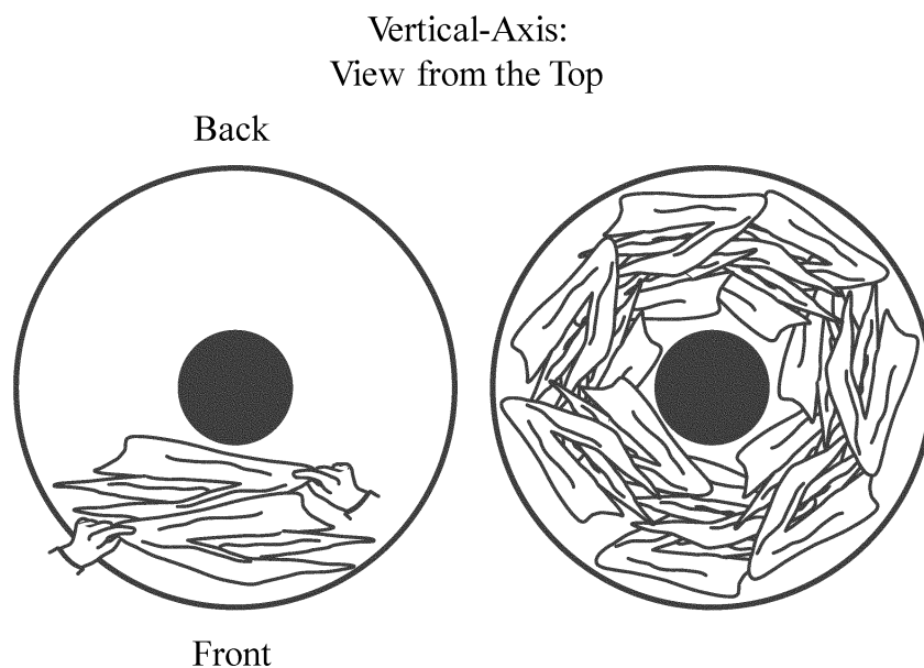
Figure 2.8.3.1—Loading Energy Test Cloths into a Top-Loading Clothes Washer
