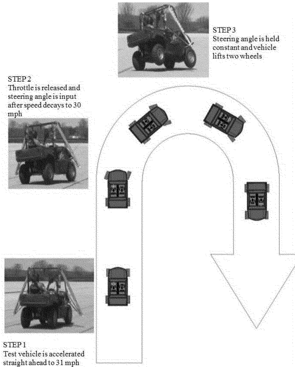
Figure 4. J-Turn Test Sequence of Events
