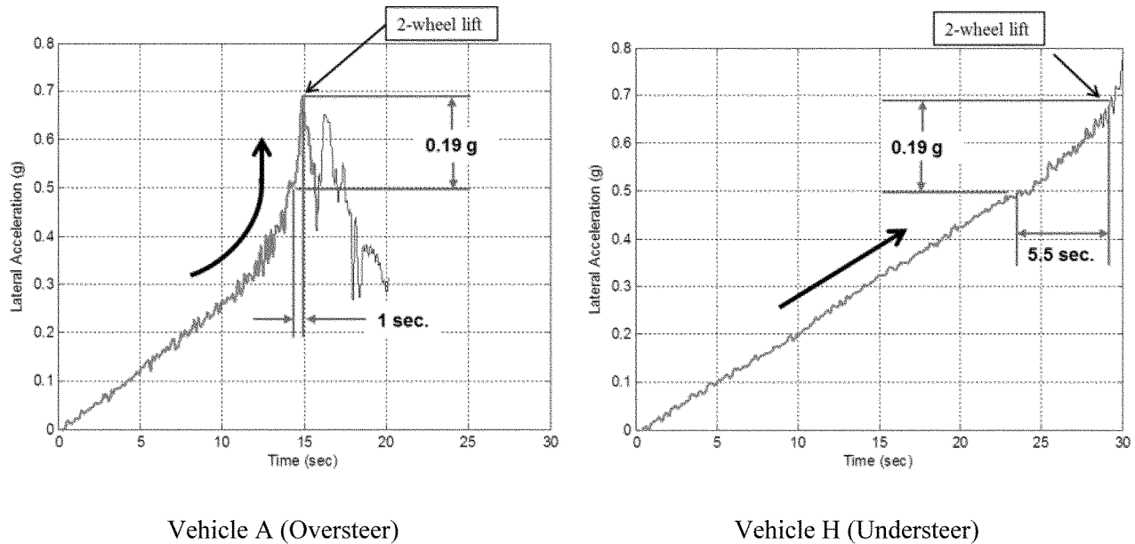
Figure 7. SIS Plots of Lateral Acceleration Gain Over Time
