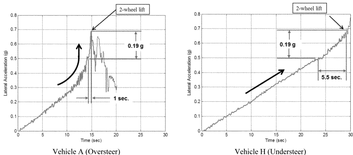
Figure 14. SIS Plots of Lateral Acceleration Gain Over Time
