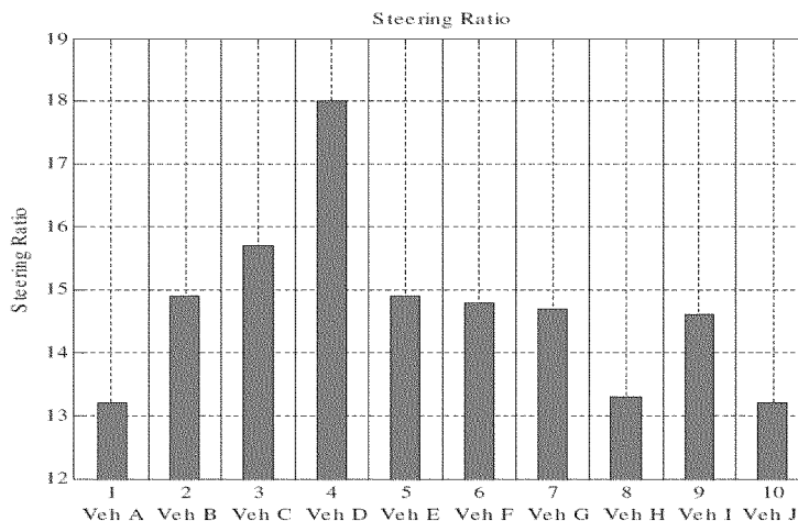
Figure 13. Steering Ratio = steering wheel input (degrees)/change in front wheel angle (degrees)
