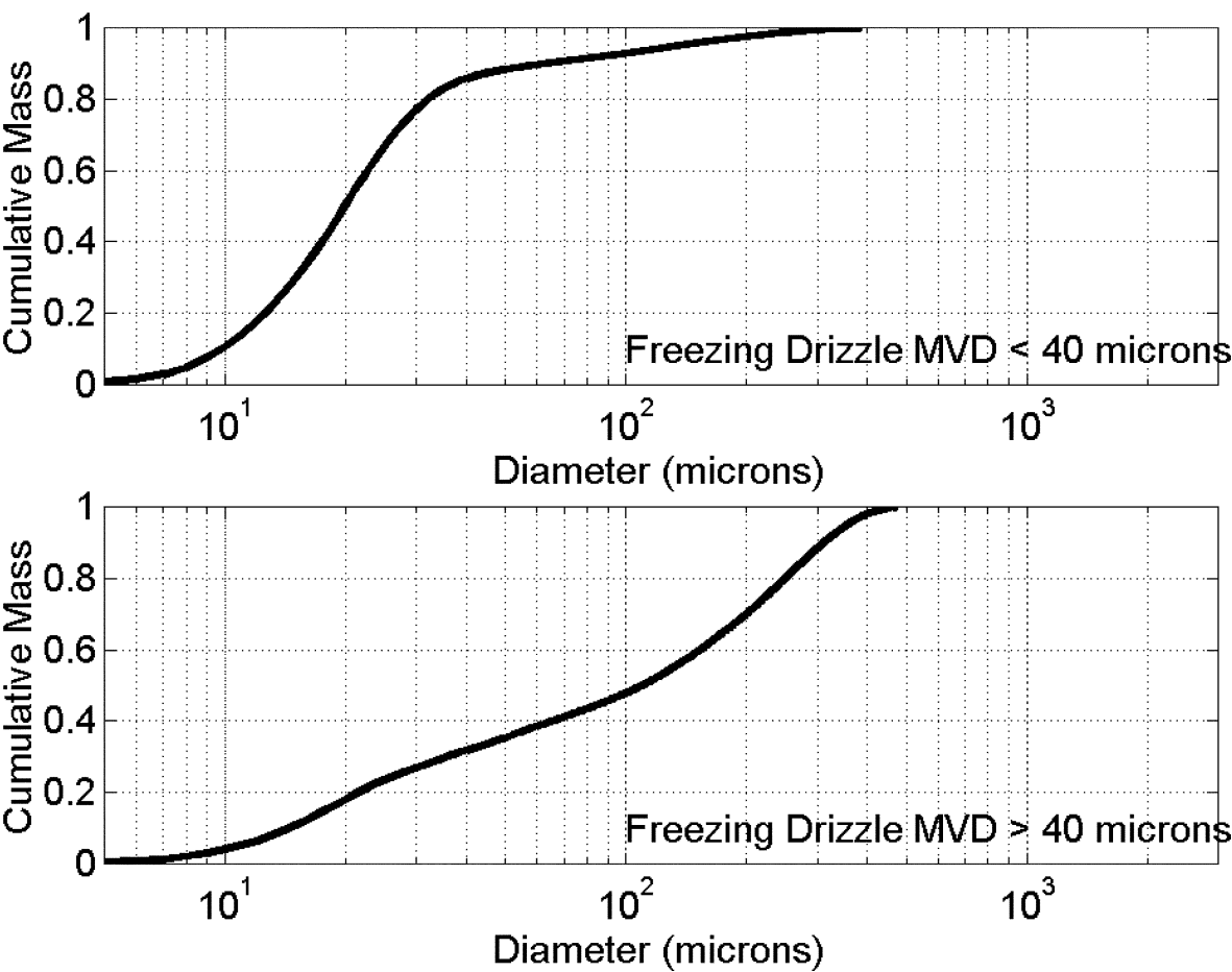
FIGURE 2 — Appendix O, Freezing Drizzle, Drop Diameter Distribution
