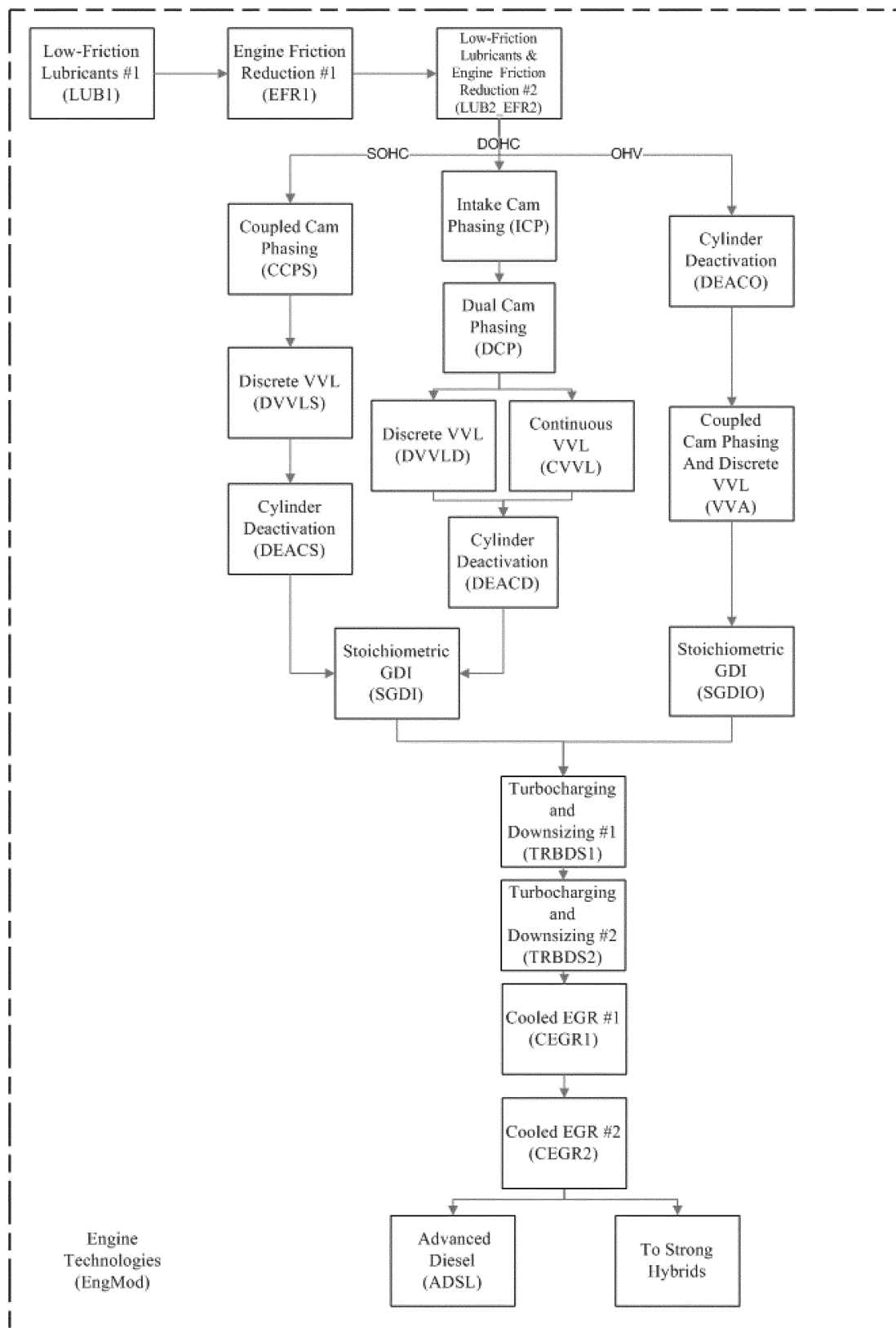
Figure IV-1 NHTSA Simplified Engine Decision Tree Used in the CAFE Model
