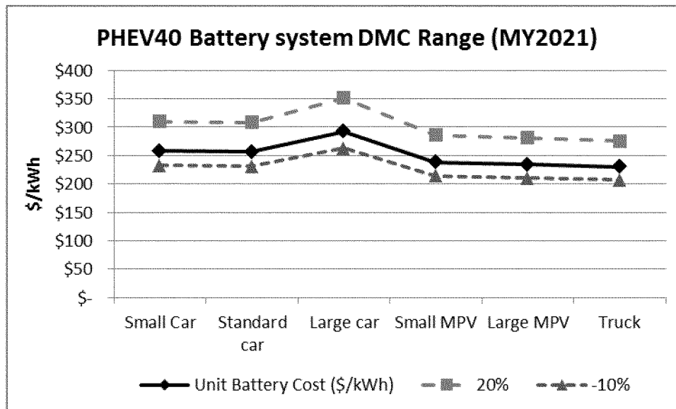
Figure IV-7 Battery System Direct Manufacture Cost (DMC) for PHEV40
