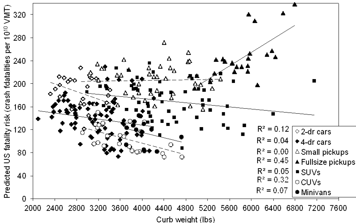
Figure II-2 _Predicted US fatality risk per VMT vs. curb weight by vehicle type, after accounting for all driver, crash, and vehicle variables except mass and footprint
