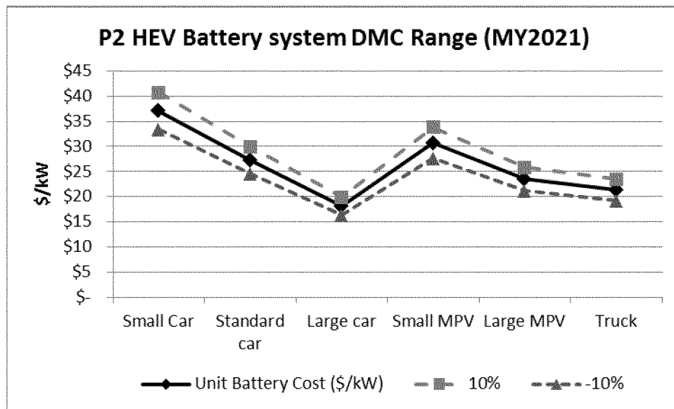
Figure IV-5 Battery System Direct Manufacture Cost (DMC) for P2 HEV
