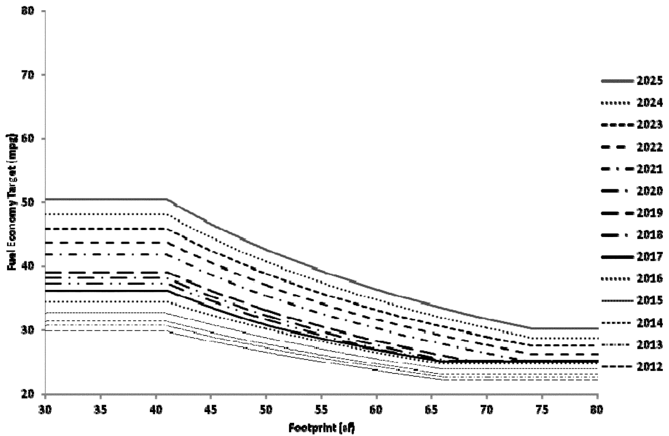
Figure I -2 CAFE Target Curves for Light Trucks
