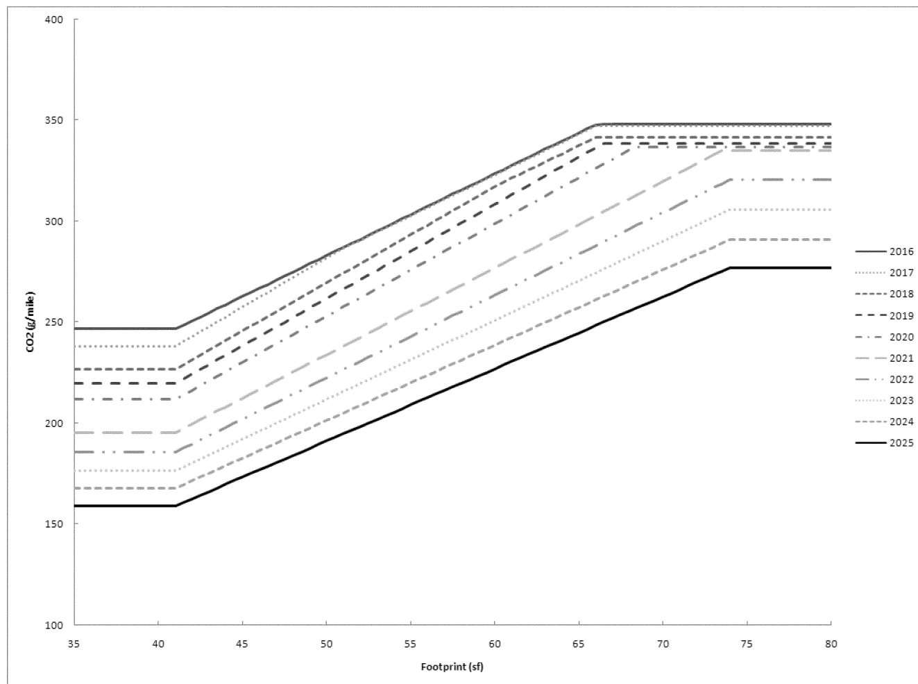
Figure I-4 CO 2 (g/mile) Light-Truck Standard Curves
