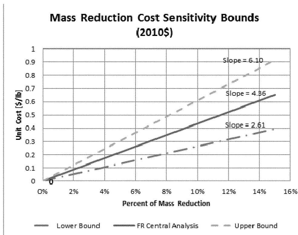
Figure IV-10 Direct Manufacturing Cost for Mass Reduction (2010$)
