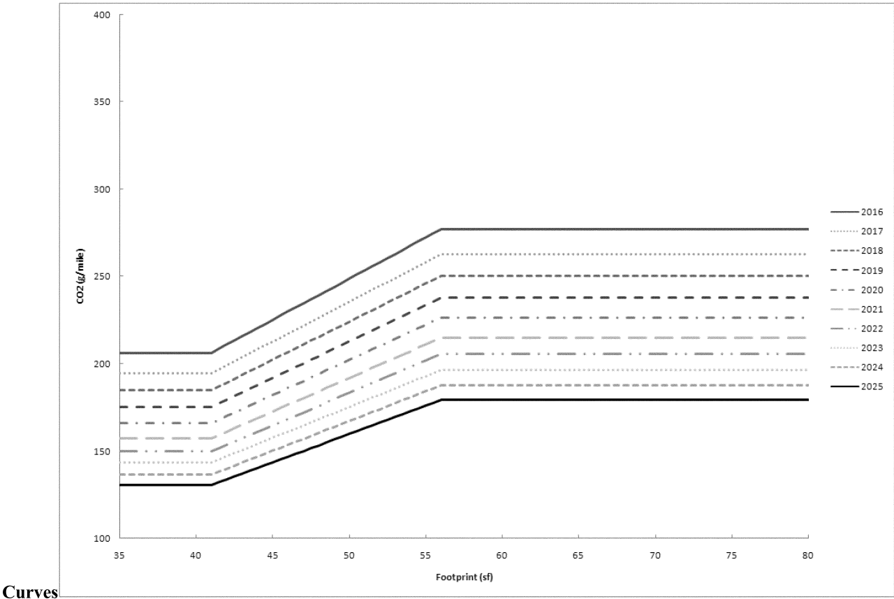
Figure I- 3 CO2 (g/mile) Passenger Car Standards
