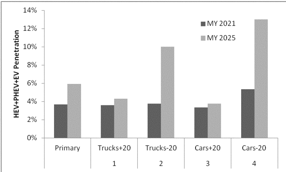
Figure III-3 HEV + PHEV + EV Penetration for Manufacturers above 500,000 Sales
