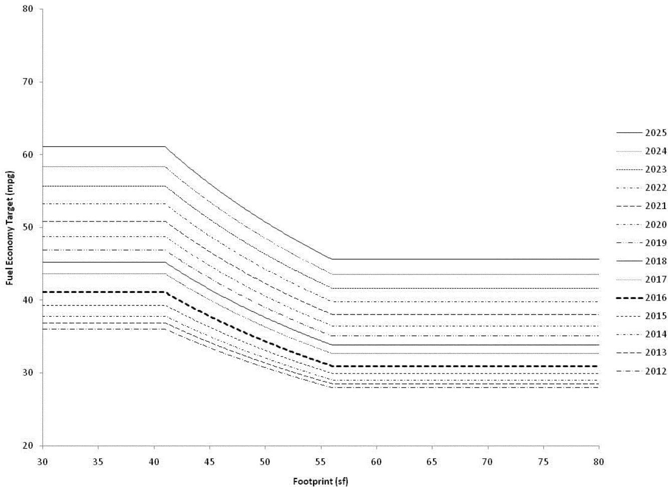
Figure I-1 CAFE Target Curves for Passenger Cars
