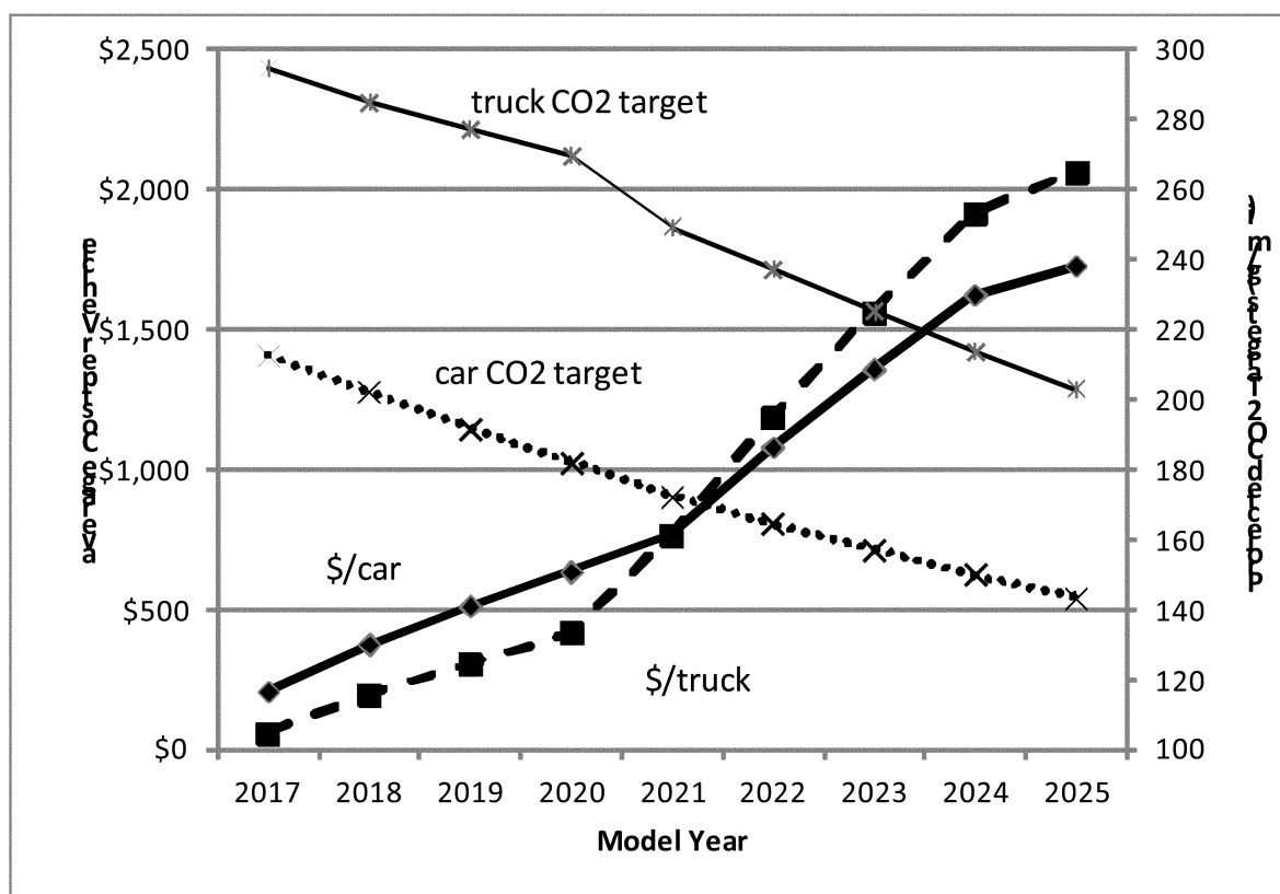
Figure III-5 Year on Year Progression of Projected (Target) CO 2 Standards and Average Cost Per Vehicle
