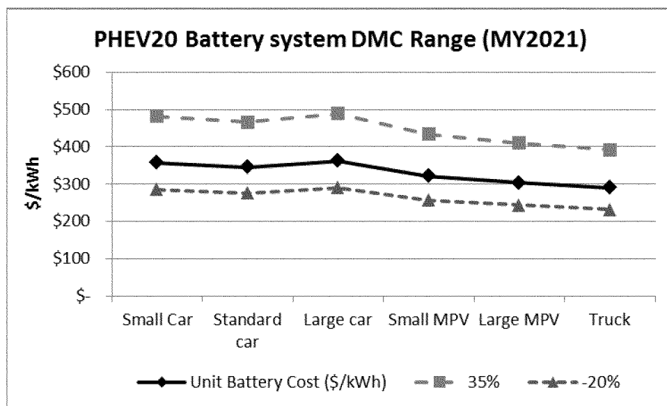
Figure IV-6 Battery System Direct Manufacture Cost (DMC) for PHEV20
