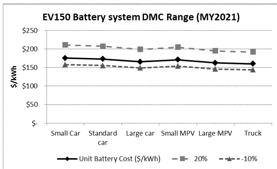
Figure IV-9 Battery System Direct Manufacture Cost (DMC) for EV150
