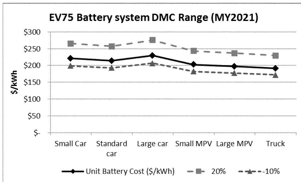
Figure IV-8 Battery System Direct Manufacture Cost (DMC) for EV75
