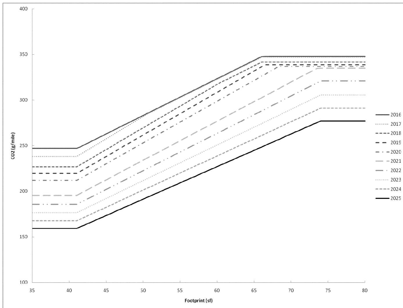
Figure III-2 –Truck Curves
