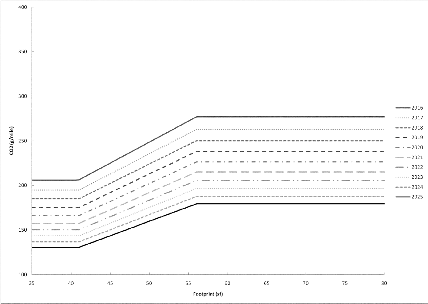
Figure III-1 Car Curves
