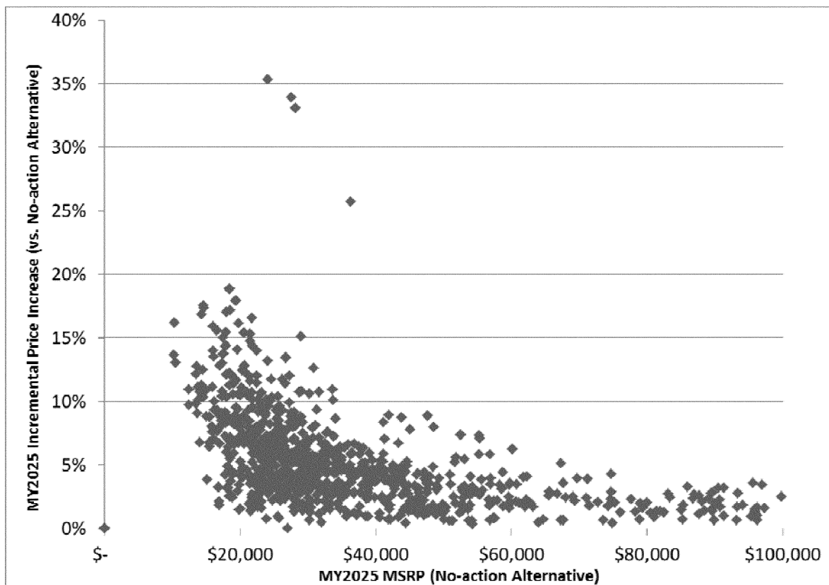
Figure IV-4 NHTSA Estimated Incremental Cost Increases in MY 2025
