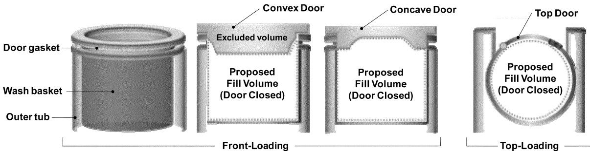
Figure III.2 Representation of Fill Volumes for the Clothes Container Capacity Measurement for Horizontal-Axis (Front-Loading and Top-Loading) Clothes Washers 11
