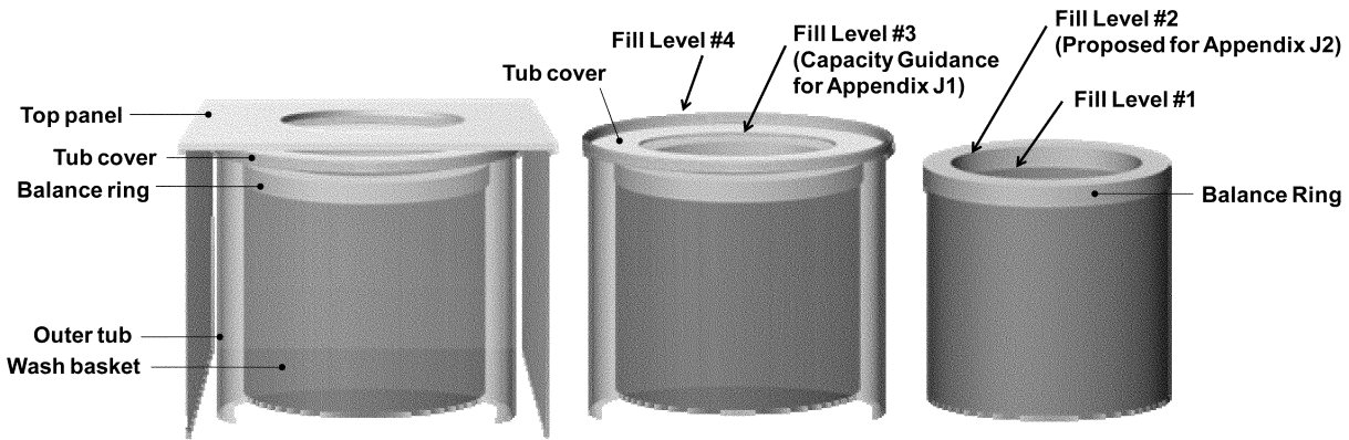
Figure III.1 Representation of Fill Levels for the Clothes Container Capacity Measurement for Vertical-Axis (Top-Loading) Clothes Washers
