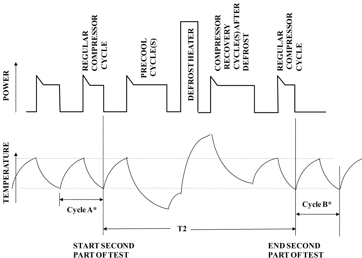
Long-time Automatic Defrost Diagram for Cycling Compressors
