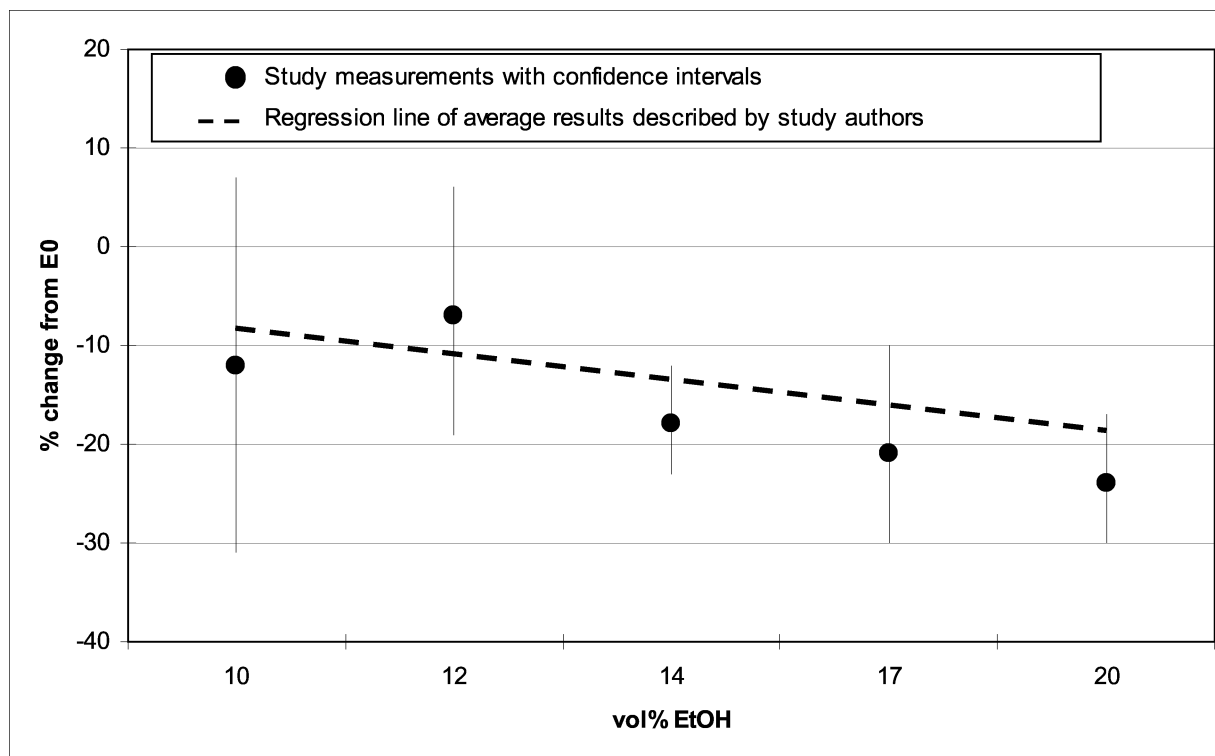
Figure V.B-1: Illustration of results of study by Guerrieri, et al for Total Hydrocarbons (THC)
