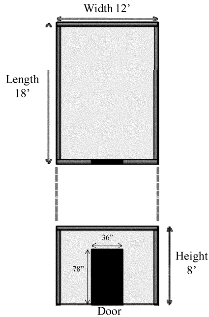
Figure 4 Geometry of Infiltration Test Unit
