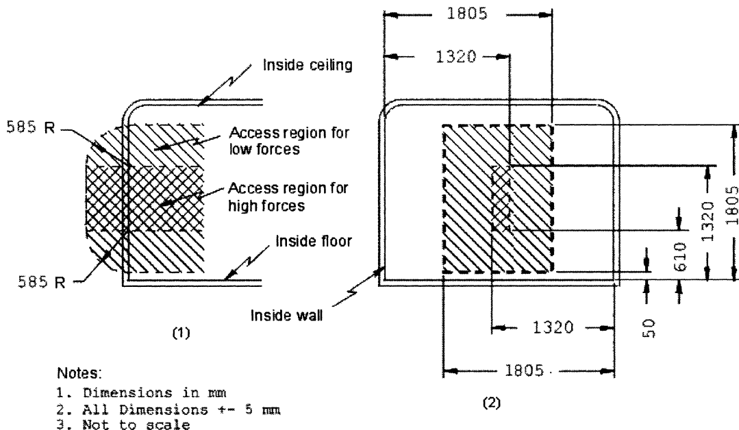
Figure 3D- REAR EMERGENCY EXIT WITHOUT REAR OBSTRUCTION
