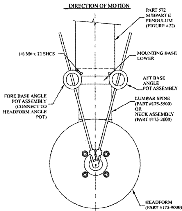
Figure U2-A NECK/LUMBAR SPINE/HEADFORM ATTACHED TO PENDULUM
