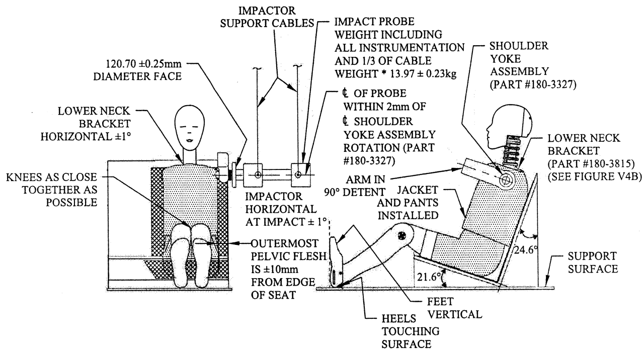
FIGURE V4-A SHOULDER IMPACT
