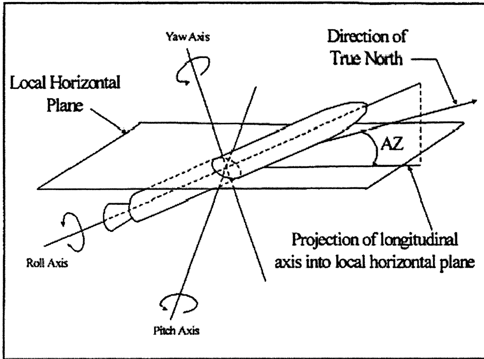
Figure A417.9-4, Illustrative Longitudinal Axis Azimuth (AZ)
