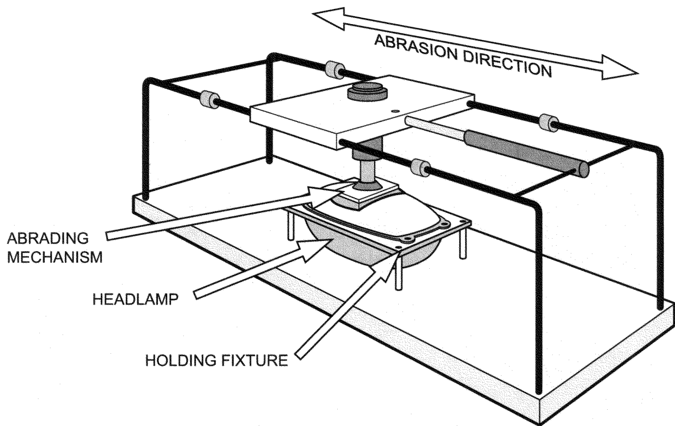
HEADLAMP ABRASION TEST FIXTURE
